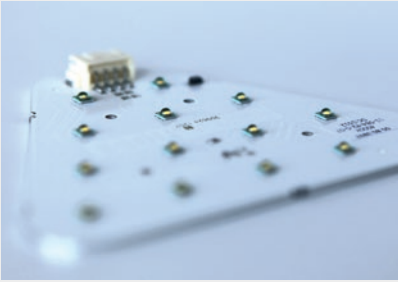
modules for street lighting
